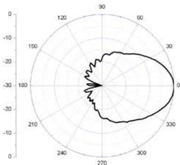
E Plane (90° )
