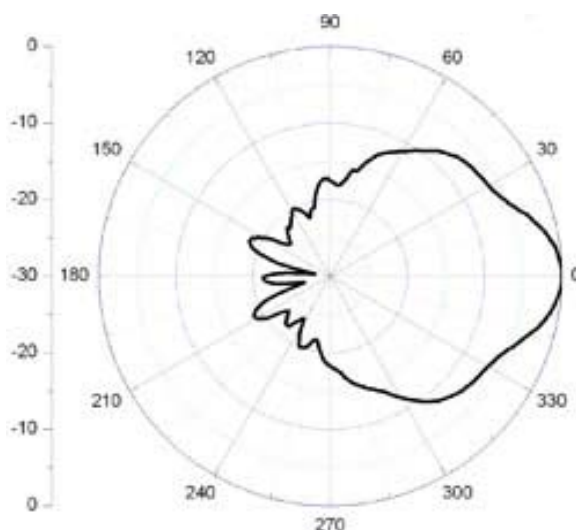
E Plane (90° )
