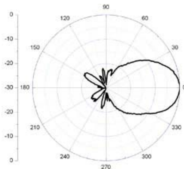
H Plane (32° )
