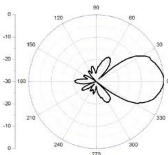
H Plane (32° )
